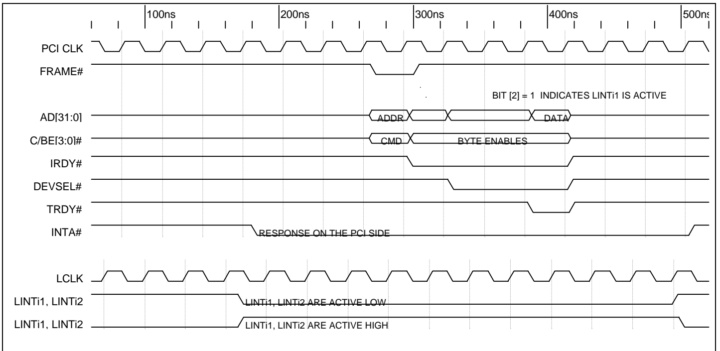
Timing Diagram 8-3. Local LINTi1# Input Asserting PCI Output INTA#
